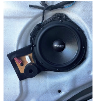
woofer in the vehicle door IVECO VI Installation situation
